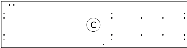
CA3590 1400x350x38mm
