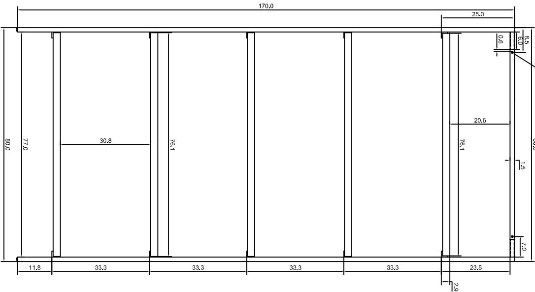
FRONT ELEVATION
