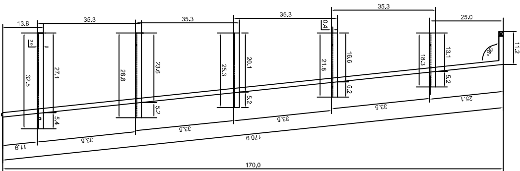
SIDE ELEVATION
