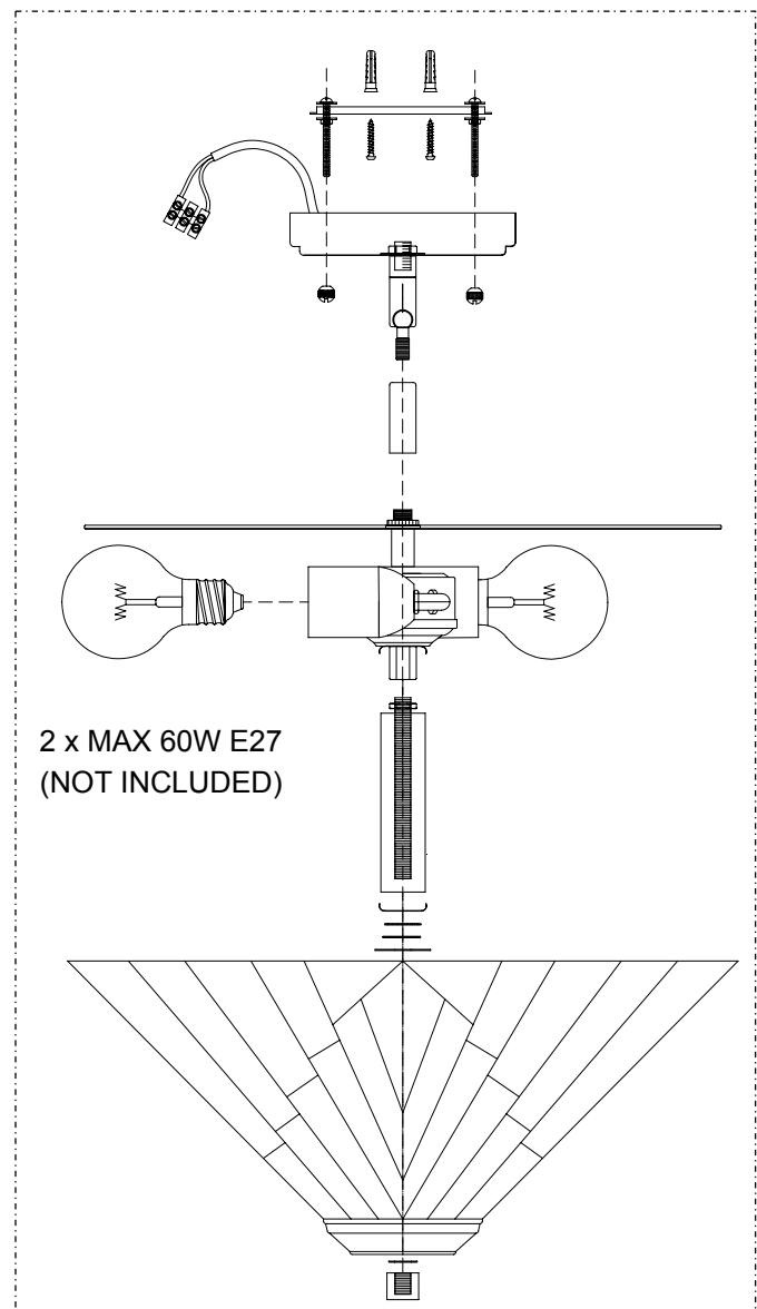
FLUSH MOUNTING
