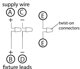
Drawing 3 - Post-Mount
