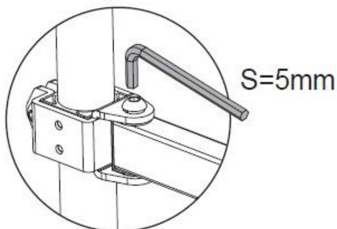
Arm Adjustment
