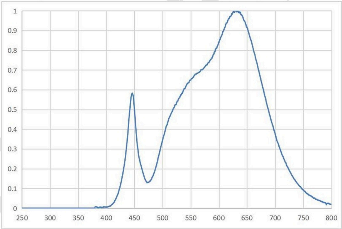
Light source 2: CCT 3000K: Chromaticity coordinates (x and y):0.440, 0.403
