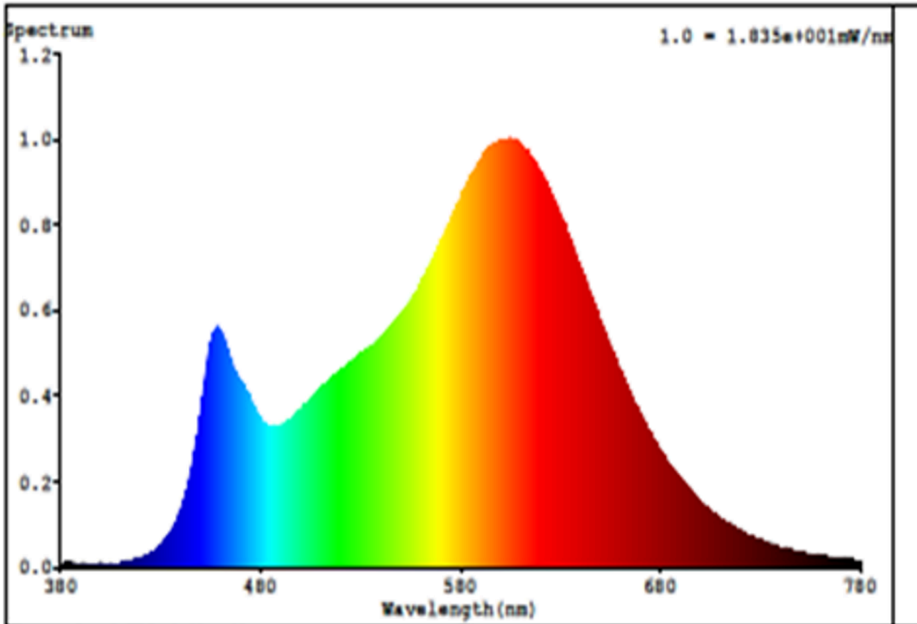
Spectral Distribution
