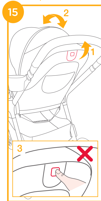
Stroller Operation
