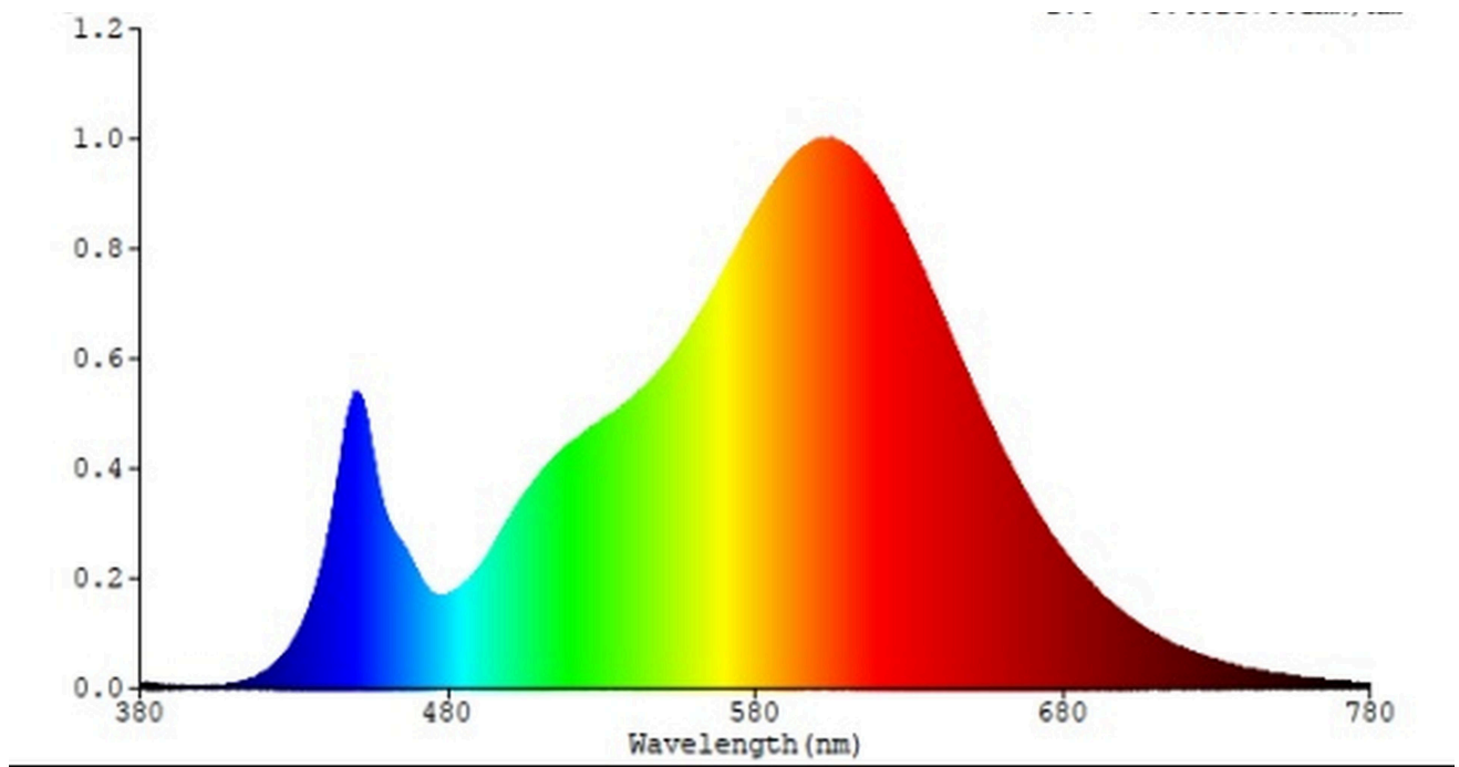
63600029-01_Light source
