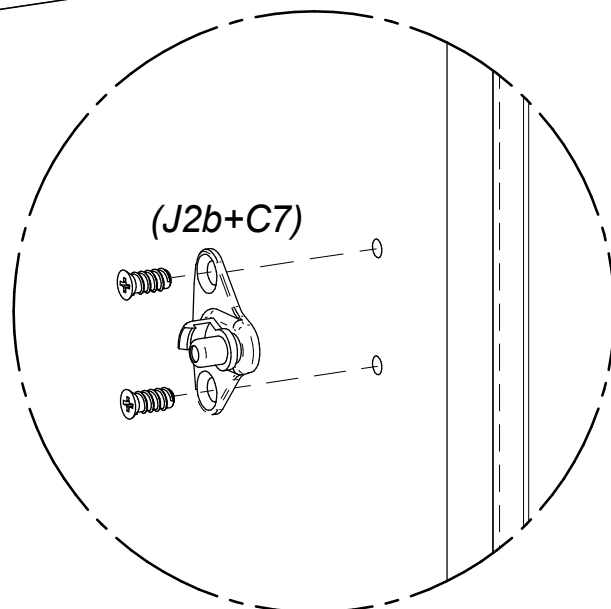
DETAIL D
