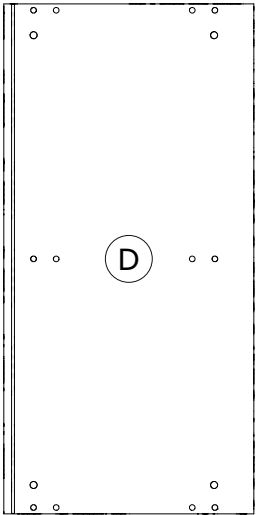
BA02535 720x353x16mm
