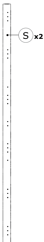
FS05280 1849x60x22mm
