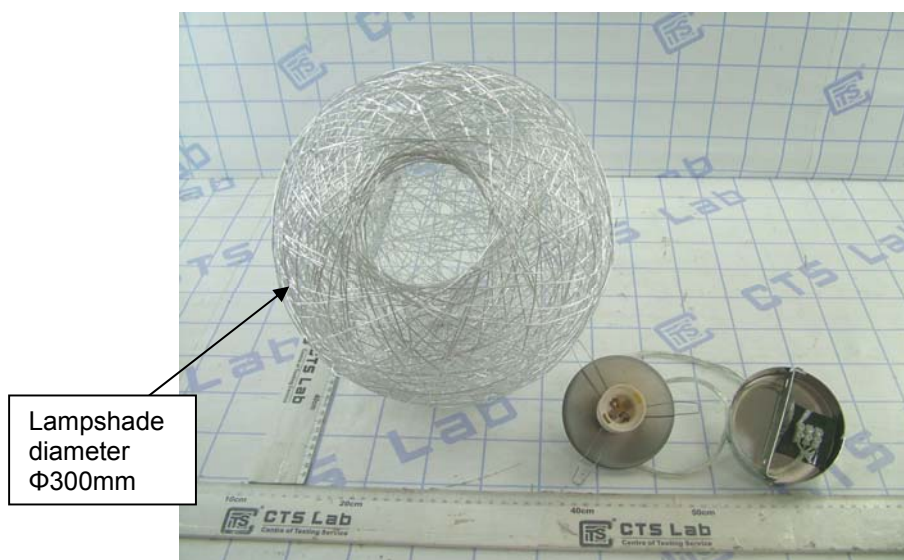
Figure 2 (Internal construction 1)
