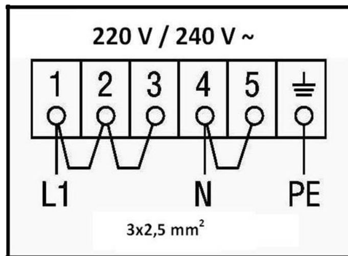
Connection diagram
