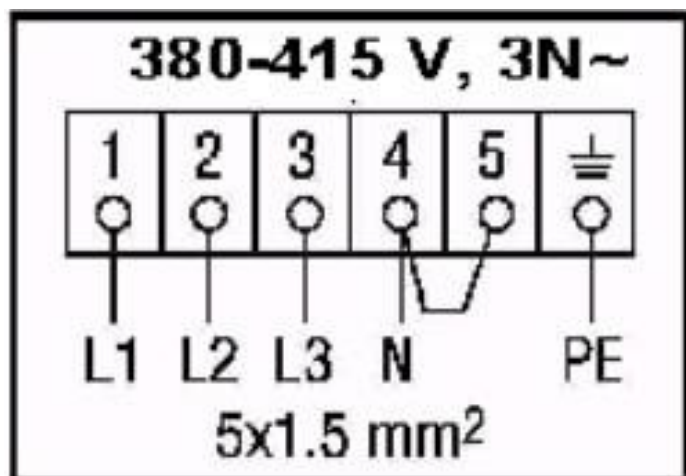
Connection diagram
