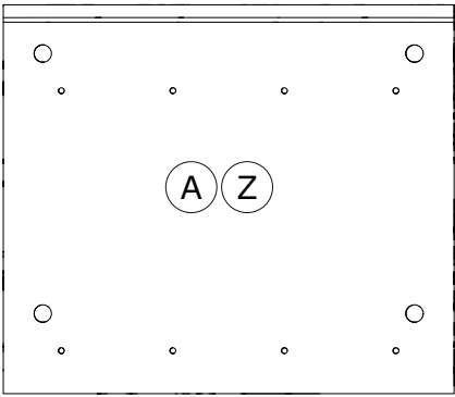
FI10327 388x335x16mm
