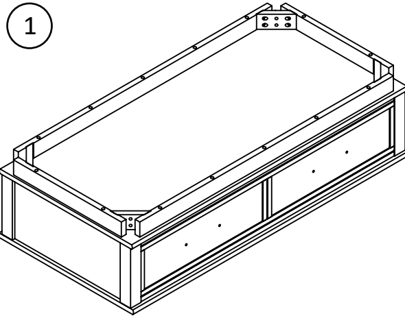
x1 T6914013010UD PRE-ASSEMBLE BODY
