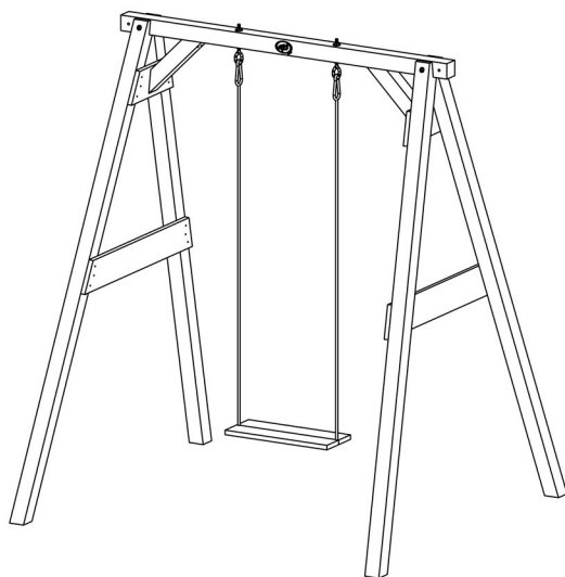
Single Swing A030.136.00
