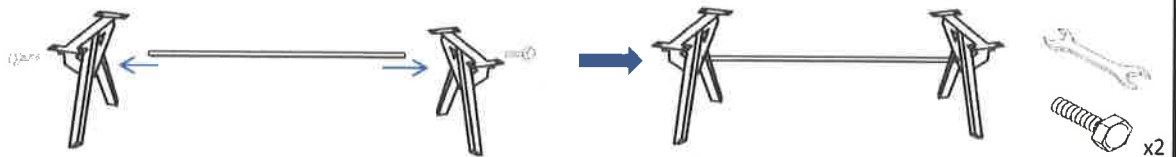
FIGURE : 1 Attach the pipe to center of the both leg with the help of bolt and spanner as shown above.
