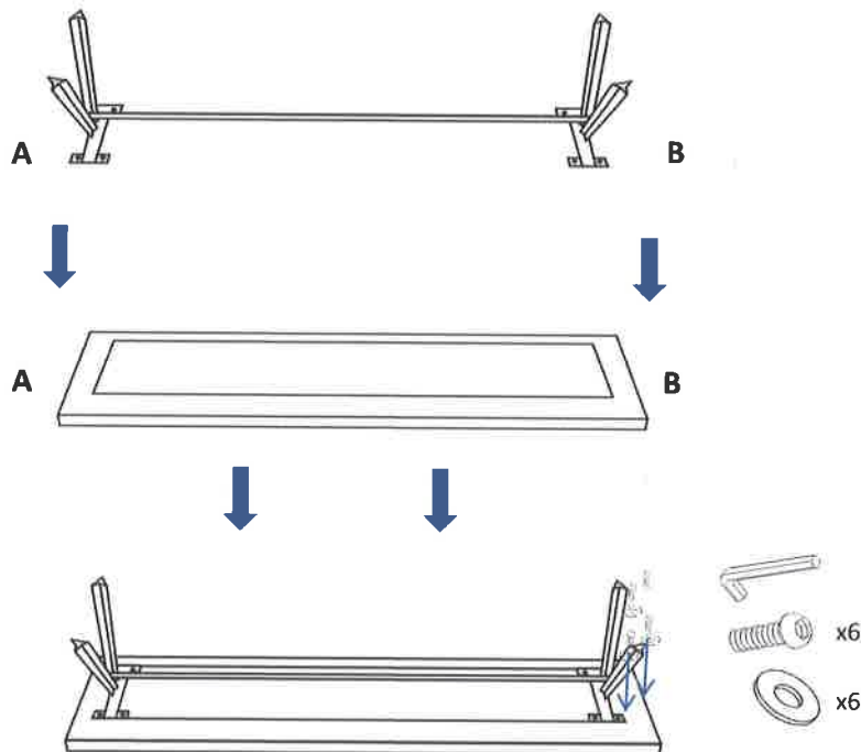
FIGURE : 2 Attach the dining base to the dining top with the help of d-nut and Allen key as shown above.
