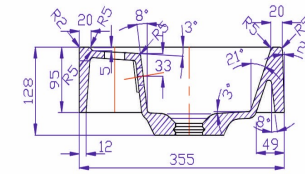
REZ B-B/ SECTION B-B
