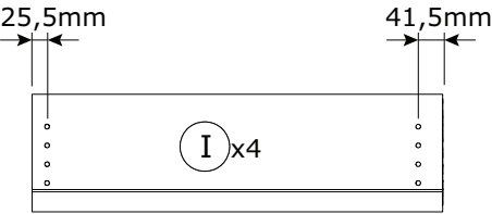
CS2802 672x200x18mm
