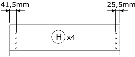
CS2800 672x200x18mm
