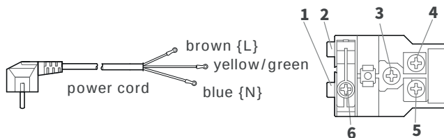
terminal box
