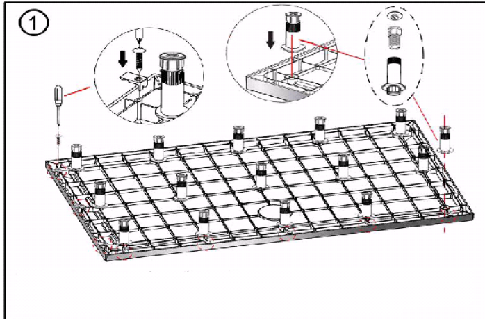
M5*12mm 8x
