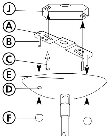
Drawing 3 - Fixture Mounting
