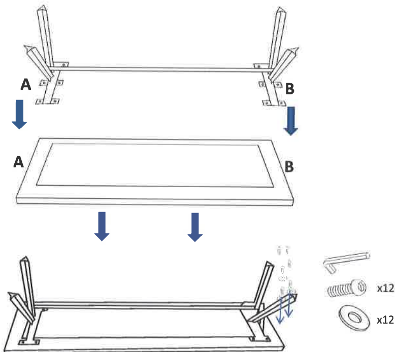
FIGURE : 2 Attach the dining base to the dining top with the help of d-nut and Allen key as shown above.
