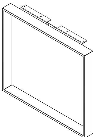
FW0691 800x690x80mm
