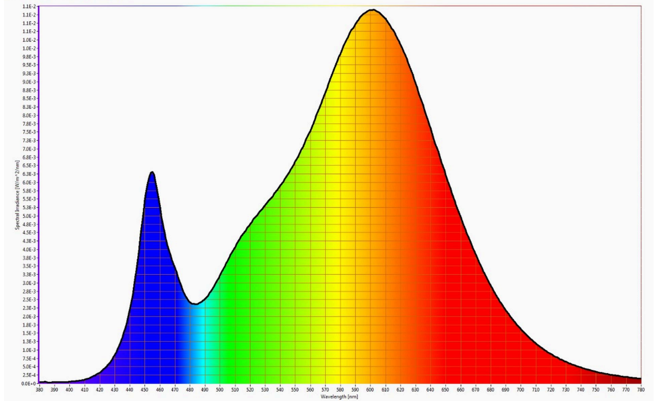
PowerSpectrum @ 1 meter Source Sensor Distance
