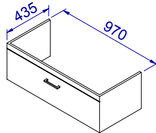
Cabinet Dimensions
