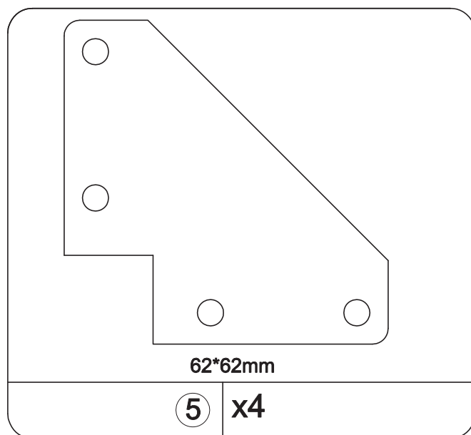
METAL PLATE TDM0044
