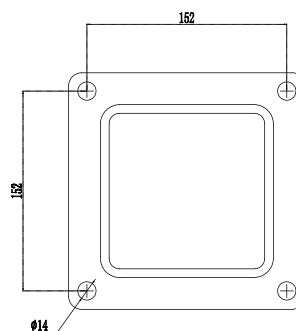
Lochabstand Bodenplatte | Hole spacing Base plate
