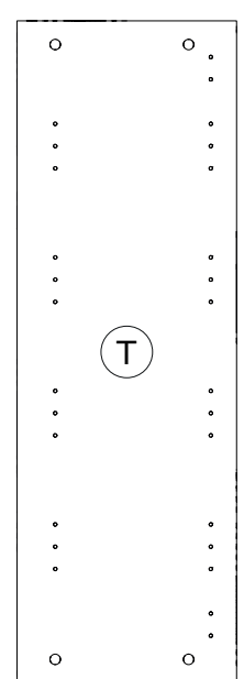
TR02695 952x316x16mm
