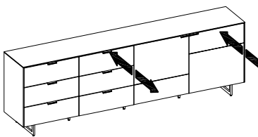
Adjust the gap between door panel and side panel
