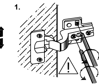
1. Unscrew 2 screws in round holes Loosen 2 screws in oval holes
