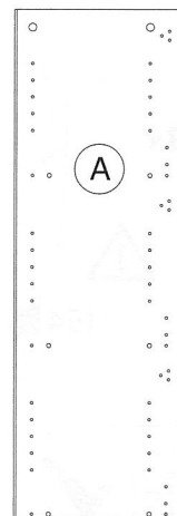
FI8511 968x327x18mm
