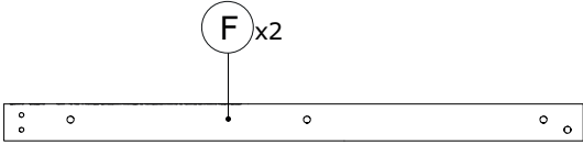
FS4766 1254x80x30mm
