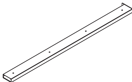
FW0379 L.=1177mm
