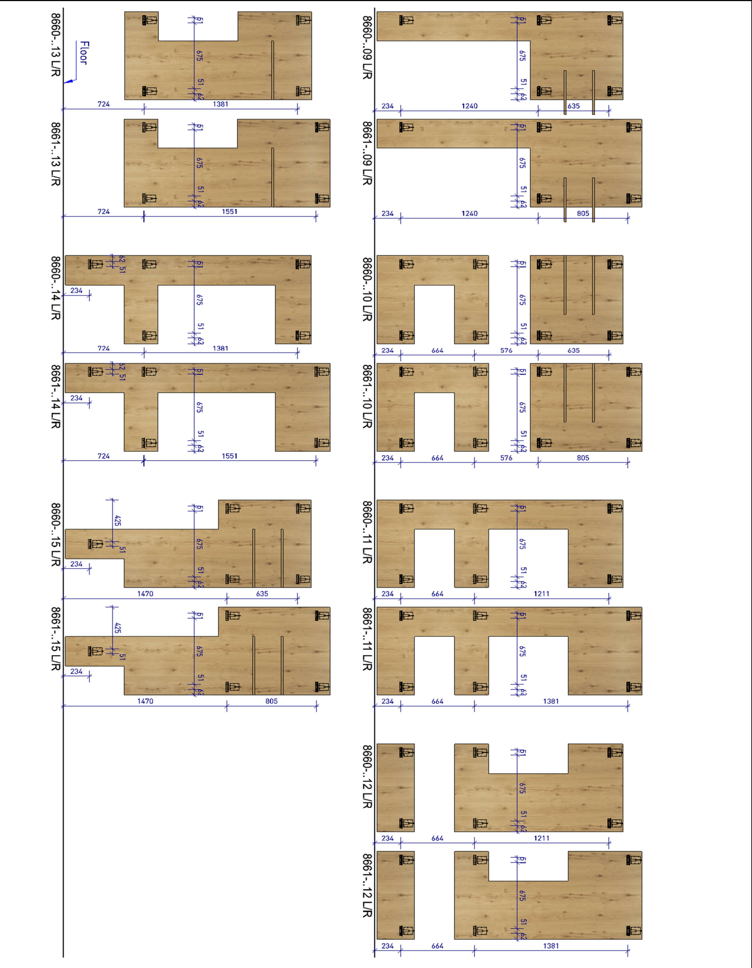
Fig. 5:Drill dimensions for suspension rails All measurements in mm!
