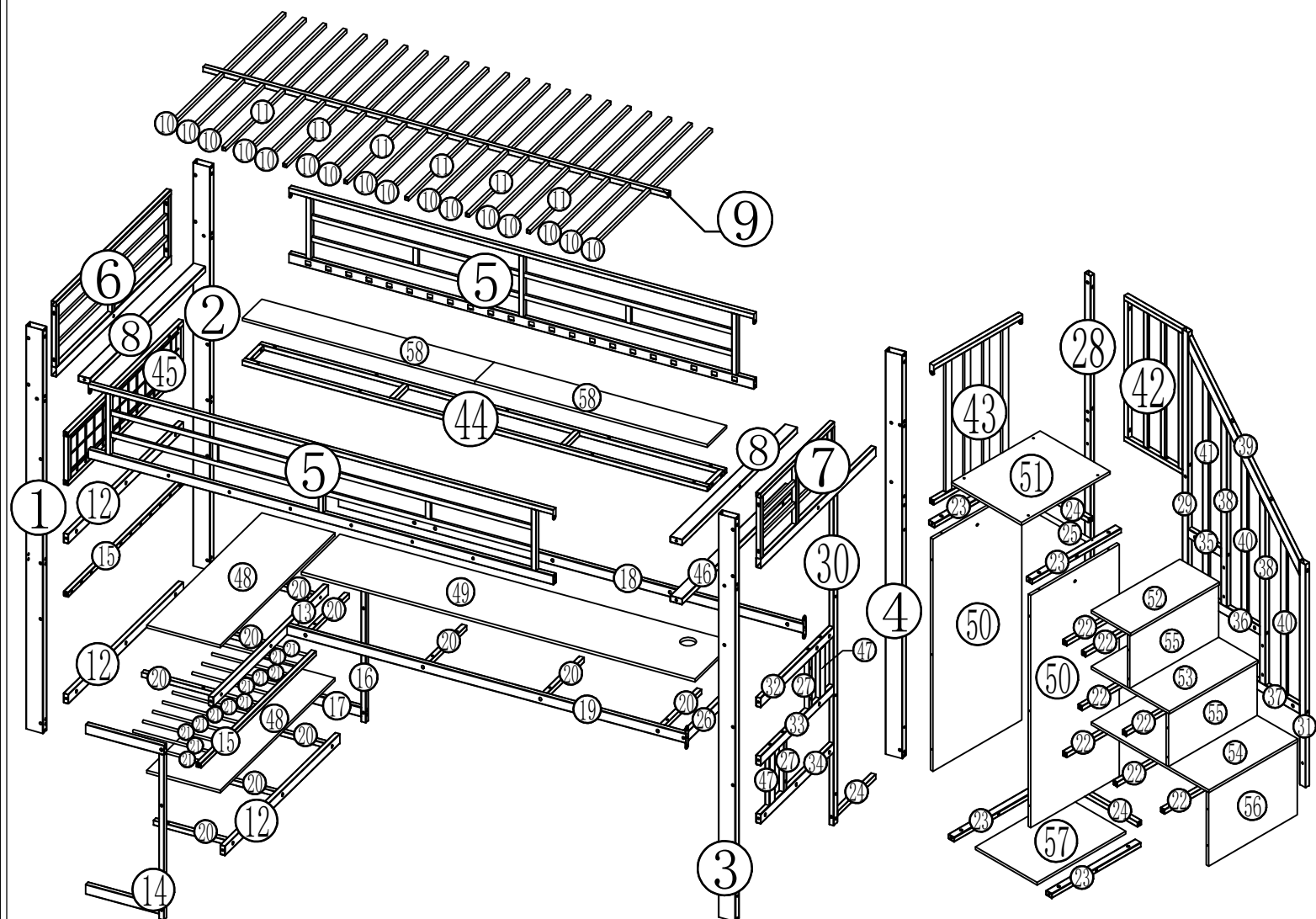
Bed parts view
